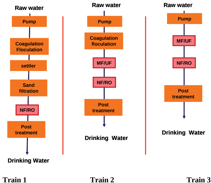
Figure 2 : Treatment trains for drinking water production
